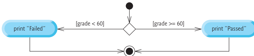
Fig. 4.5 | if...else double-selection statement UML activity diagram.
